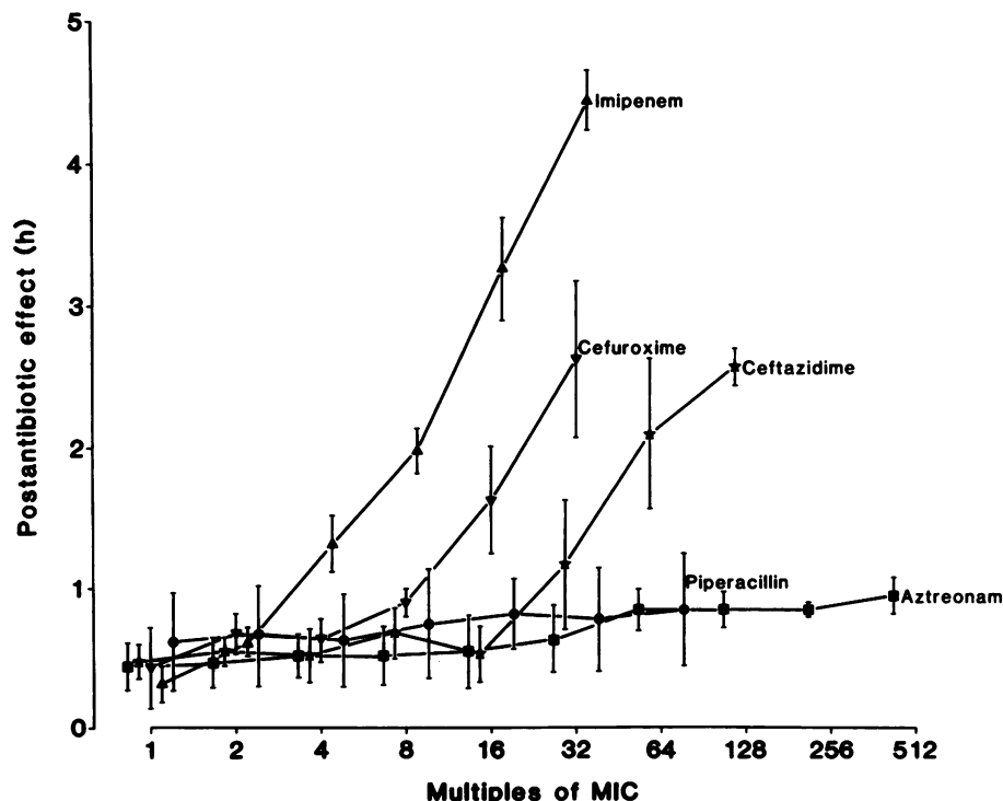
FIG. 2. PAEs of aztreonam, ceftazidime, cefuroxime, imipenem, and piperacillin on E. coli ATCC 25922 as determined by bioluminescence at different concentrations (expressed as multiples of the MIC). Mean values of the pooled results of three experiments are shown. Vertical bars denote standard deviations.
