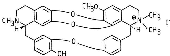
22 Coccoline methiodide S,S
