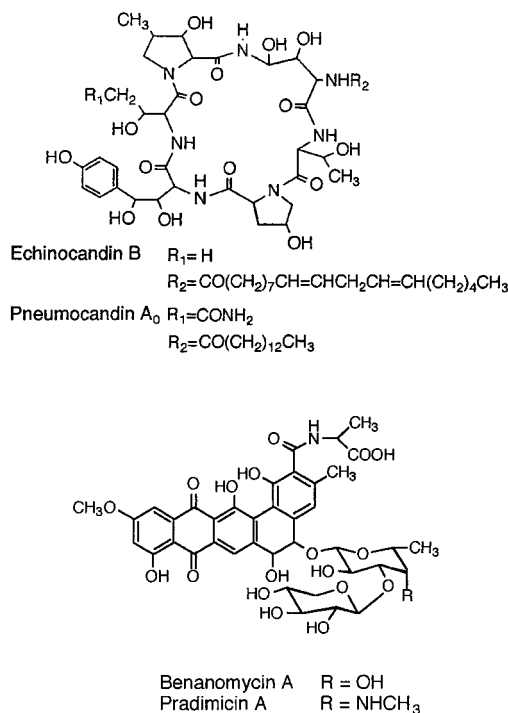
FIG. 3. Structures of some promising antifungal prototypes.
