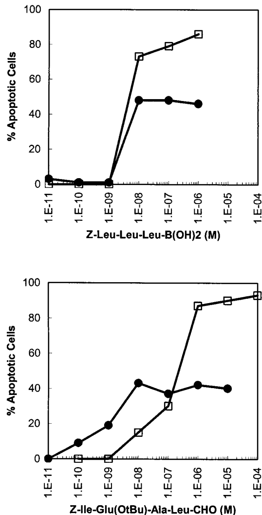
FIG. 1. Effects of Z-Leu-Leu-Leu-B(OH) 2 and Z-Ile-Glu(OtBu)-Ala-Leu-CHO on inducing apoptosis in T. brucei and human cells. TC221 bloodstream forms (●) and HL-60 cells (□) were incubated with various concentrations of the proteasome inhibitors. After 24 h of culture, cells were stained with propidium iodide and analyzed with a fluorescence-activated cell sorter. Cells from the sub-G 0 /G 1 peak were counted as apoptotic cells. The percentages of apoptotic cells were calculated in relation to the respective controls in the absence of proteasome inhibitor. Data points represent mean values from three independent experiments. The standard errors were typically less than 10%. 1.E-11 to 1.E-04, 10 -11 to 10 -4 .
