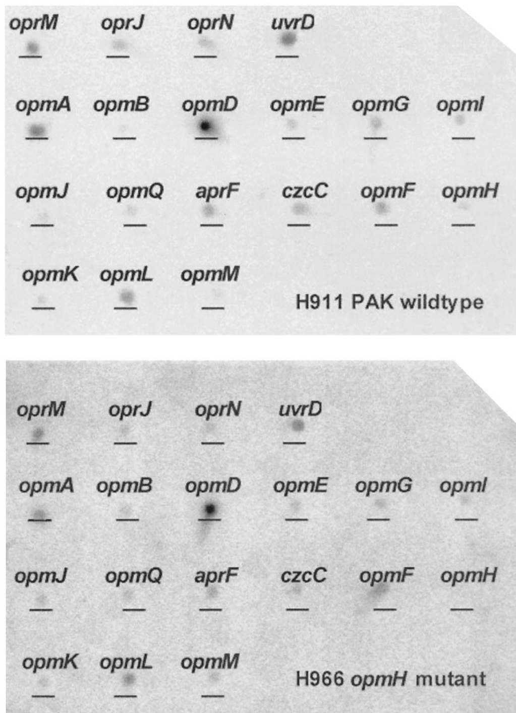
FIG. 3. Comparison of expression of OprM homolog genes in wild-type PAK (H911) (top panel) and the oprH mutant (H966) (bottom panel) by using mini-microarrays. RNA isolated from each strain was reverse transcribed to cDNA, radiolabeled with [ \alpha - ^{32} P]dCTP, and hybridized to a nylon membrane containing 10-ng spots of 600-bp internal fragments corresponding to each of the OprM homologs. Spot densitometry revealed the expected absence of oprH expression as well as 1.9- and 2-fold downregulation of oprG and opml expression, respectively.
