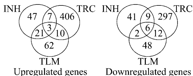
FIG. 1. Overlap of genes regulated by isoniazid, thiolactomylin, or triclosan treatment of M. tuberculosis . Numbers within the sectors indicate the total numbers of genes regulated uniquely or in common by either 1× or 5× MIC treatment of each drug at either 2 or 6 h ( P < 0.001 ). INH, isoniazid; TLM, thiolactomylin; TRC, triclosan.
