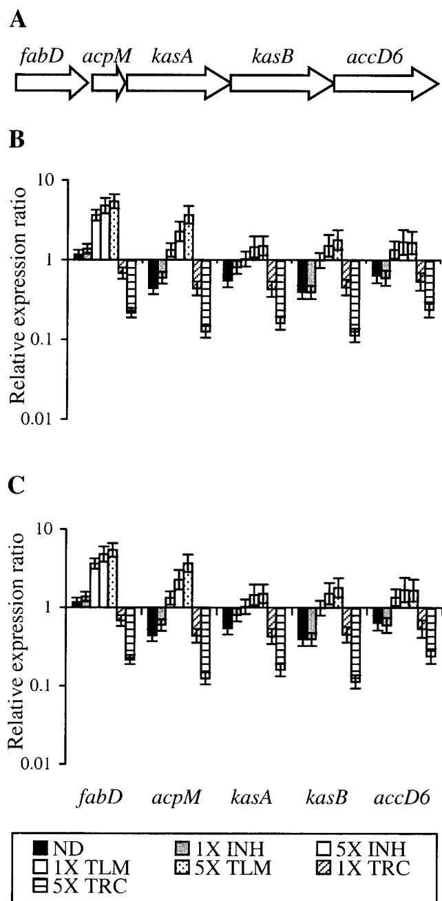
FIG. 3. Response of the kas operon to isoniazid, thiolactomyacin, or triclosan treatment as measured by QRT-PCR. (A) Schematic representation of the kas operon in the M. tuberculosis H37Rv genome. Ratio between the number of cDNA copies detected in each sample relative to the time zero control by QRT-PCR at 2 h (B) and 6 h (C) is represented. Each value is the average of two biological replicates, each analyzed in duplicate. INH, isoniazid; TLM, thiolactomyacin; TRC, triclosan.
