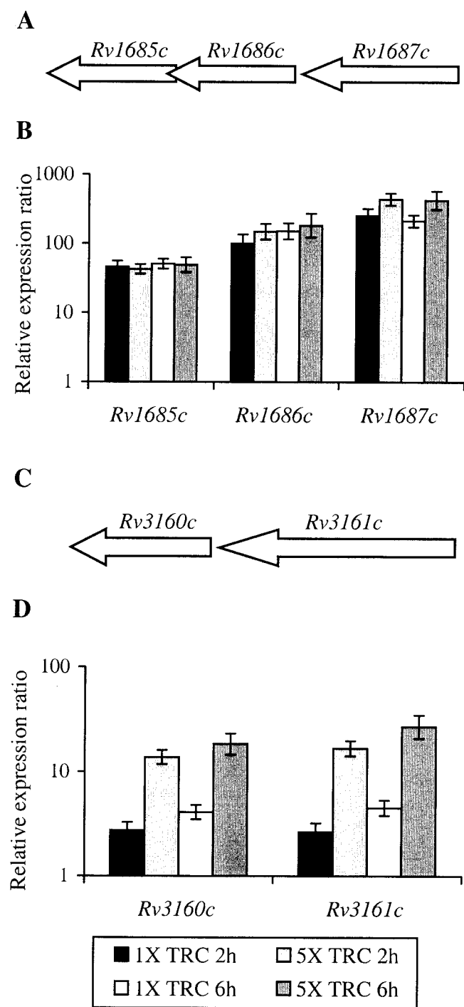
FIG. 4. Genes induced by triclosan treatment of M. tuberculosis as measured by QRT-PCR. Organization of Rv1685c to Rv1687c (A) and Rv3160c to Rv3161c (C) in the M. tuberculosis H37Rv genome. Ratio between the number of cDNA copies detected in each sample relative to the time zero control by QRT-PCR for Rv1685c to Rv1687c (B) and Rv3160c to Rv3161c (D). Each value is the average of two biological replicates, each analyzed in duplicate. TRC, triclosan.
