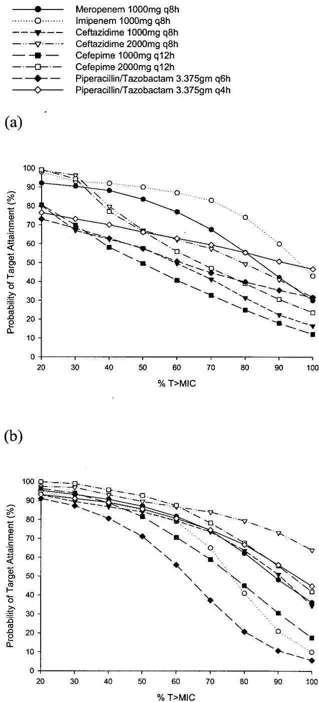
FIG. 2. Probabilities of target attainment at different free drug % T>MIC targets for \beta -lactams against A. baumannii (a) and P. aeruginosa (b).
