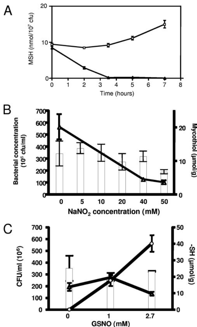
FIG. 2. MSH pool in M. smegmatis is decreased by exposure to NO. (A) MSH levels in M. smegmatis mc 2 155 in 0.9% saline solution decreased by continuous exposure to gNO. Organisms were exposed to 400 ppm gNO (triangles) or medical air (squares) for 7 h. The amount of MSH decreased steadily to almost zero in less than 3.5 h on gNO exposure. (B) MSH levels in M. smegmatis mc 2 155 decreased with exposure to the NO donor sodium nitrite, while bacterial viability remained relatively unaffected. M. smegmatis mc 2 155 was grown to log phase in Middlebrook 7H9 media supplemented with 0.05% Tween and 1% glucose (pH 5.5), diluted to 0.5 optical density units at 600 nm in the same medium, and treated with various concentrations of sodium nitrite for 2 hours. Numbers of CFU (bars) and MSH levels (triangles) are shown. (C) MSH levels in M. smegmatis mc 2 155 decreased with exposure to the NO donor GSNO, while viability remained unaffected. M. smegmatis mc 2 155 was grown to log phase in Middlebrook 7H9 media supplemented with 0.05% Tween and 1% glucose, diluted to 0.5 optical density units at 600 nm with the same medium, and treated with various amounts of GSNO for 2 h. CFU/ml (bars), GSH levels (circles), and MSH levels (triangles) are shown. Each data point represents the mean \pm standard error for four independent measurements.
