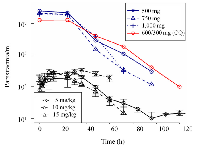
FIG 3 Parasitemia in mefloquine-treated, Plasmodium -infected volunteers (this study) or malaria patients. Blue lines, treatment in earlier studies with mefloquine; red lines, treatment with chloroquine (CQ; 600/300 mg) (27, 28).
